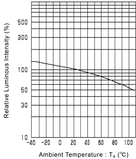
Relative Luminous Intensity vs. Ambient Temperature
