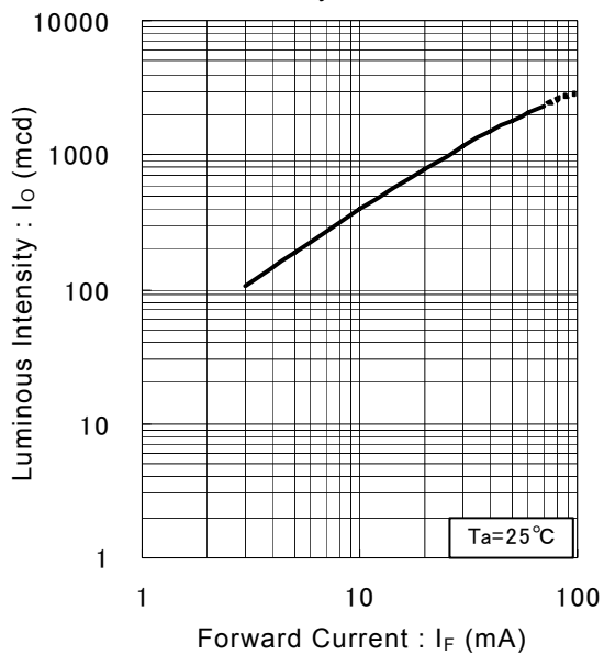
Luminous Intensity vs. Forward Current
