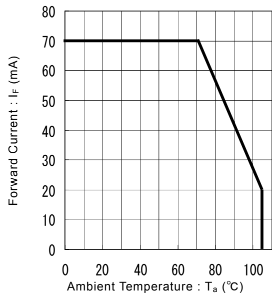
Forward Current vs. Ambient Temperature
