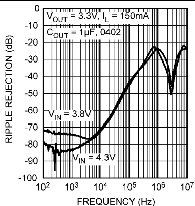
Figure 3. Power Supply Rejection Ratio
