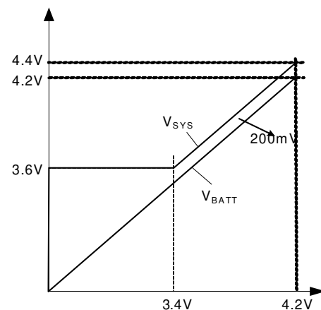
Figure 2: SYS Regulation Output
