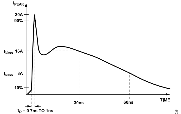
Figure 45. IEC 61000-4-2 ESD Waveform (8 kV)
