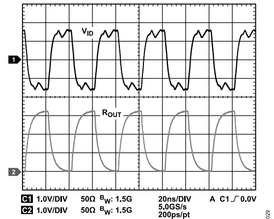
Figure 32. Receiver Propagation Delay (Oscilloscope Plot) at 50 Mbps, |V ID | ≥ 1.5 V
