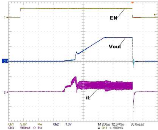
FIGURE 10. SOFT-START
