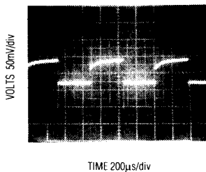
0mA TO 100mA LOAD V CC = +9V, V OUT = -5V 2N2907 OUTPUT TRANSISTOR
