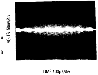
0mA TO -40mA LOAD V CC = +9V, V OUT = -5V ZTX749 OUTPUT TRANSISTOR
