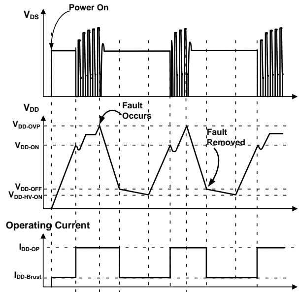
Figure 33. Auto-Restart Mode Operation
