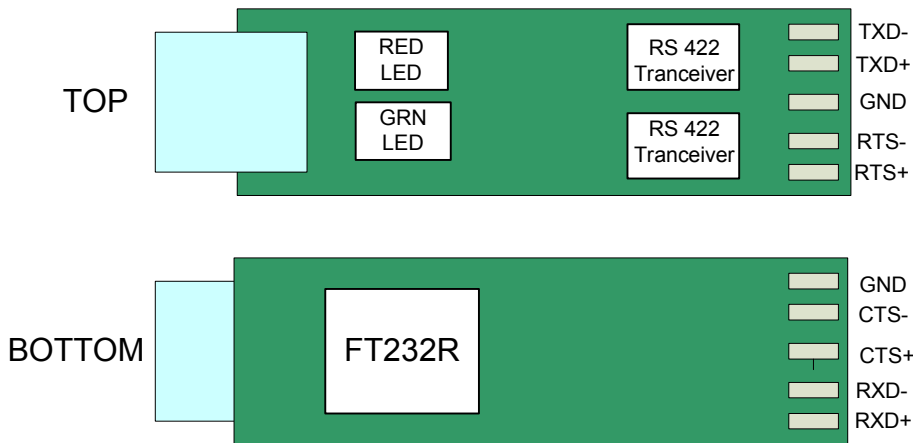
USB-RS422-PCB REV 2
