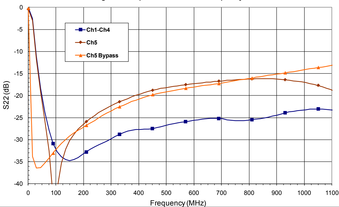
Figure 6: Output Return Loss vs. Frequency
