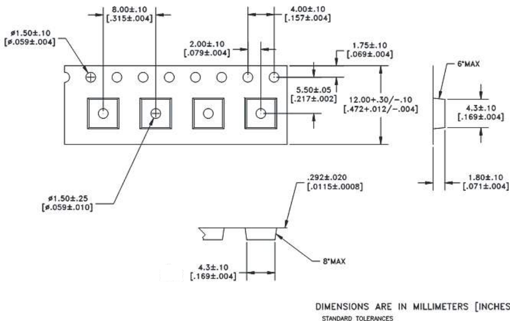
Figure 16: Tape & Reel Packaging
