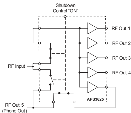
Figure 1: Functional Block Diagram “ON” Mode
