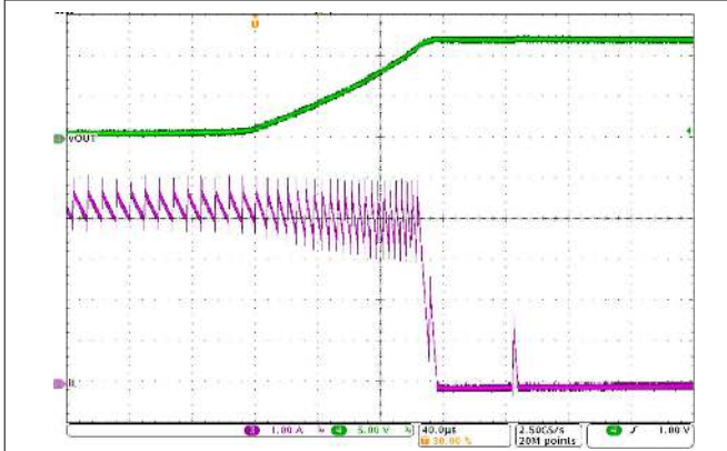
V_{IN} = 48\text{ V} V_{OUT} = 12\text{ V} Load = 0 A to Short
