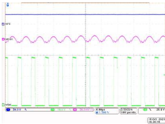
V_{IN} = 48\text{ V} V_{OUT} = 12\text{ V} I_{OUT} = 3.5\text{ A}
