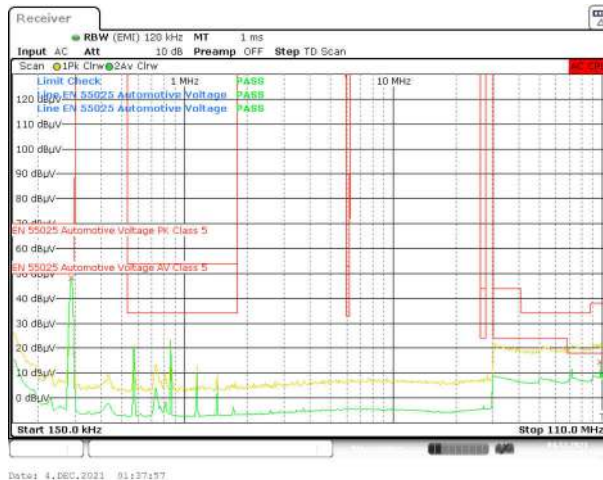
V_{IN} = 48\text{ V} V_{OUT} = 12\text{ V} I_{OUT} = 3.5\text{ A}
