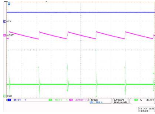
V_{IN} = 48\text{ V} V_{OUT} = 12\text{ V} I_{OUT} = 200\text{ mA}
