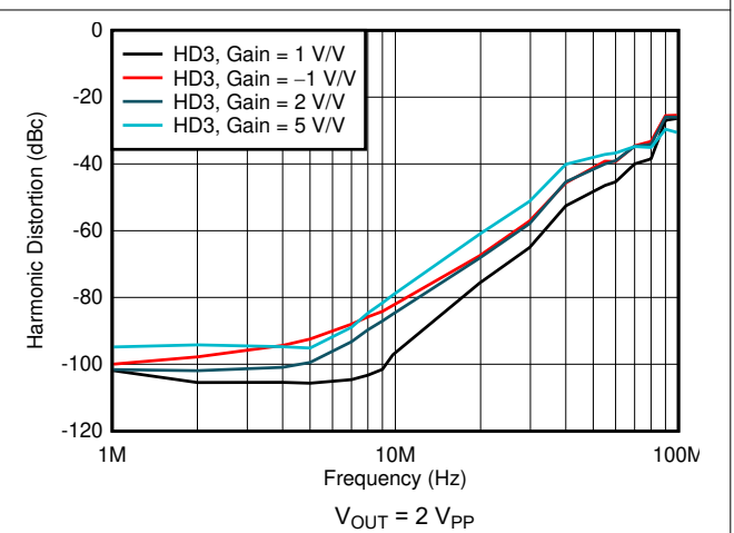
Figure 7-16. Harmonic Distortion (HD3) vs Gain
