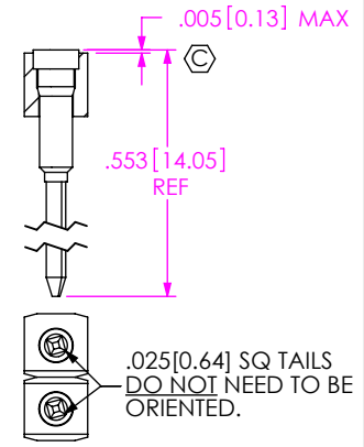
FIG 18 TERMINAL STYLE -L-2
