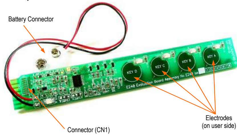
Figure 1 — Board Layout
