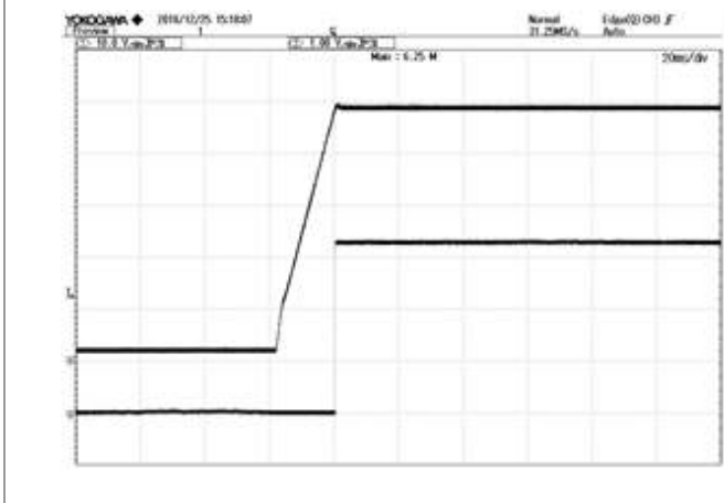
Figure 9: PG voltage vs. Vout @ Vin=220Vac, 0Alout TOP: Vout, 10V/div, 20mS/div BOTTOM: PG, 1V/div, 20mS/div
