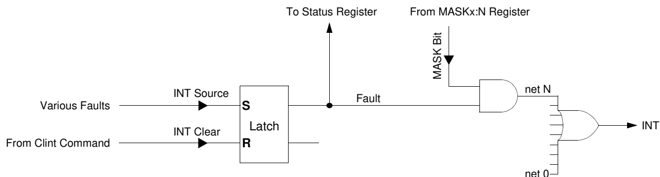
Figure 15. Interrupt Handling
