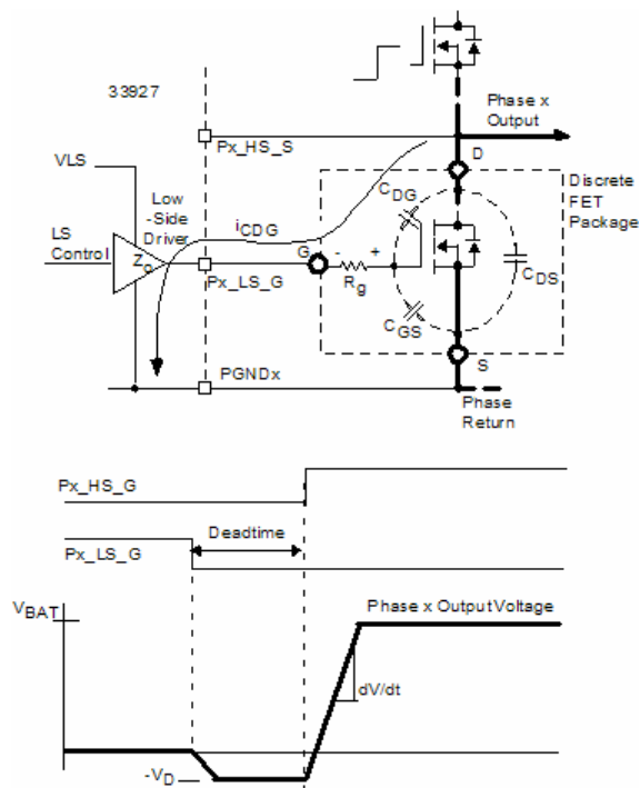
Figure 12. Positive DV/dt Transient
