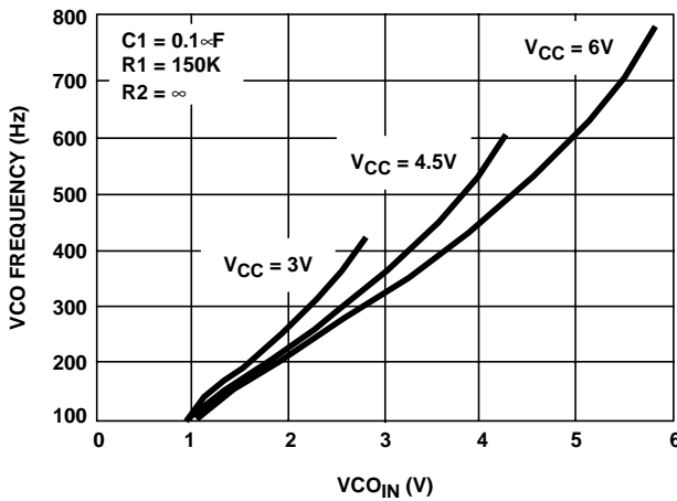
FIGURE 20. HC7046A TYPICAL VCO FREQUENCY vs VCO IN (R1 = 150kΩ, C1 = 0.1nF)
