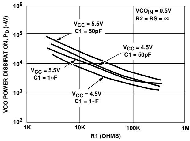
FIGURE 44. HCT7046A VCO POWER DISSIPATION vs R1 (C1 = 50pF, 1nF)
