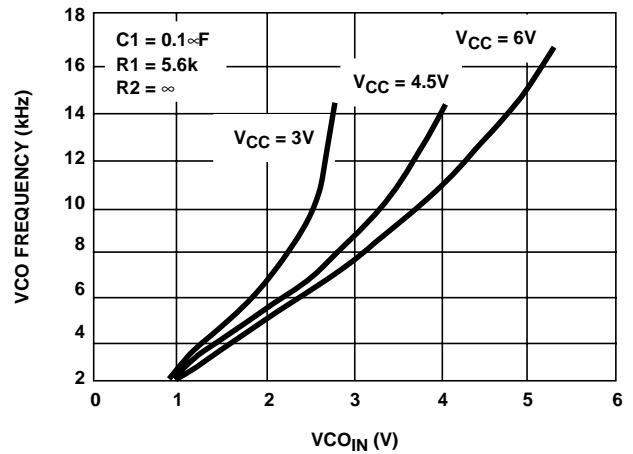
FIGURE 21. HC7046A TYPICAL VCO FREQUENCY vs VCO IN (R1 = 5.6kΩ, C1 = 0.1nF)
