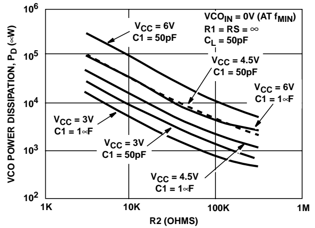
FIGURE 45. HC7046A VCO POWER DISSIPATION vs R2 (C1 = 50pF, 1nF)
