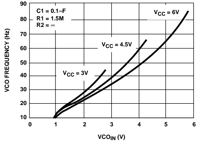
FIGURE 19. HC7046A TYPICAL VCO FREQUENCY vs VCO IN (R1 = 1.5MΩ, C1 = 0.1nF)
