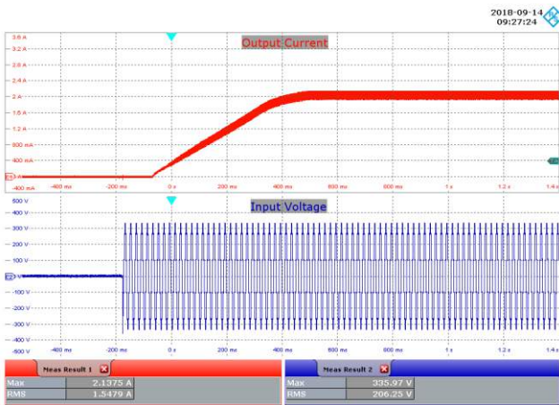
Figure 57 – 230 VAC, 36 V LED, Output Rise. Upper: I_{OUT} , 400 mA / div. Lower: V_{IN} , 100 V / div., 200 ms / div.
