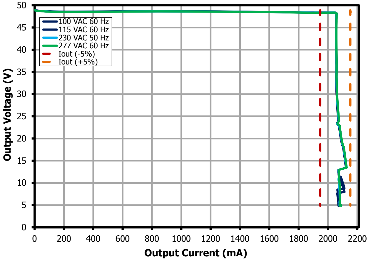
Figure 28 – CV/CC Curve.
