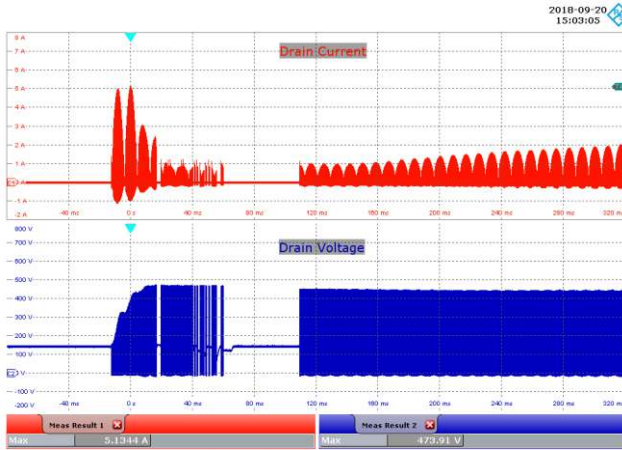
Figure 75 – 100 VAC, 48 V LED Load. Upper: I_{DRAIN} , 1 A / div. Lower: V_{DRAIN} , 100 V / div., 40 ms / div.
