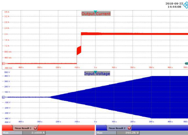
Figure 150 – Brown-in Test at 0.5 V / s. Ch1: I_{OUT} , 400 mA / div. Ch2: V_{IN} , 100 V / div. Time Scale: 100 s / div.
