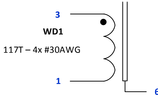
Figure 16 – PFC Inductor Electrical Diagram.
