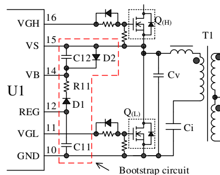
Figure 8-16. Bootstrap Circuit
