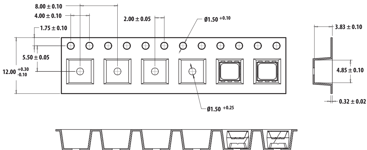
Figure 14. Carrier Tape Dimension
