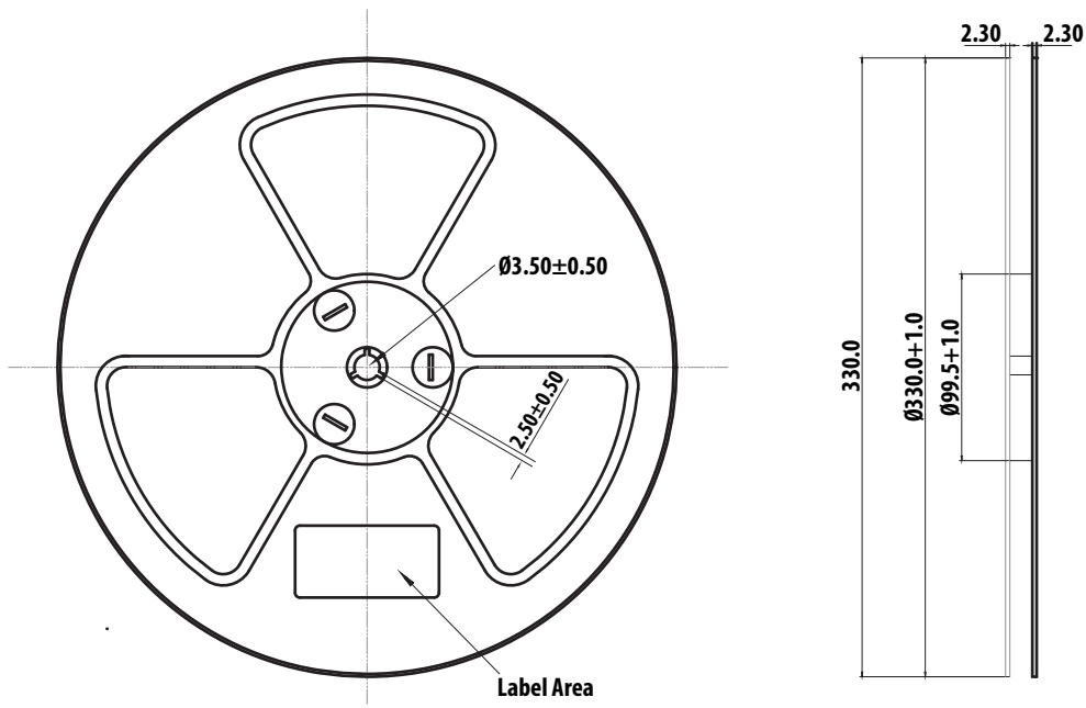
Figure 15. Reel Dimension
