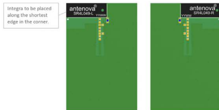
Horizontal placement
