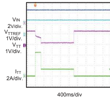
Source Over Current Protection V_{DDQ}=V_{REF}=2.5V , V_{TT}=1.25V
