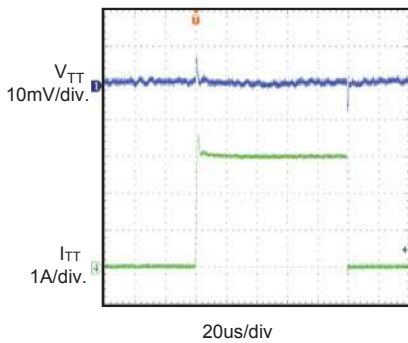
Source Load Transient V_{DDQ}=V_{REF}=1.8V , V_{TT}=0.9V
