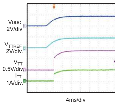
Power Ramp Up V_{DDQ}=V_{REF}=1.8V , V_{TT}=0.9V
