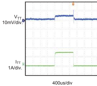
Sink Load Transient V_{DDQ}=V_{REF}=2.5V , V_{TT}=0.9V , V_{SINK}=1.8V
