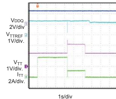
Sink Over Current Protection V_{DDQ}=V_{REF}=2.5V , V_{TT}=1.25V , V_{SINK}=2.5V
