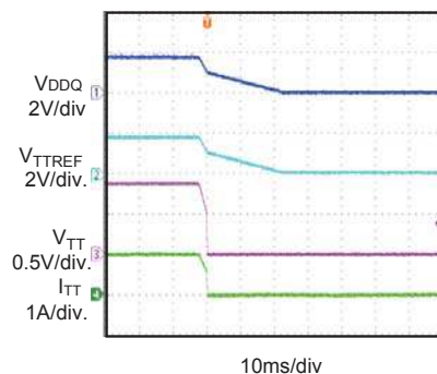
Startup Through Down V_{DDQ}=V_{REF}=1.8V , V_{TT}=0.9V
