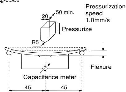
Fig.2 (in mm)
