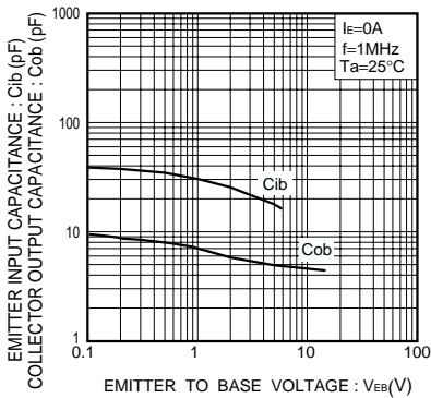
Fig.7 Collector output capacitance vs. collector-base voltage Emmitter input capacitance vs. emitter-base voltage
