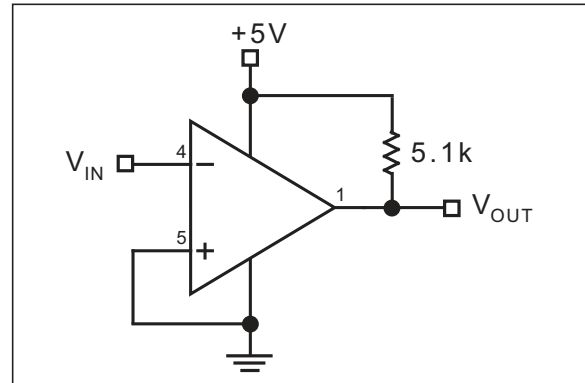
FIGURE 2-4: Output Response Time vs. Overdrive (Test Circuit).
