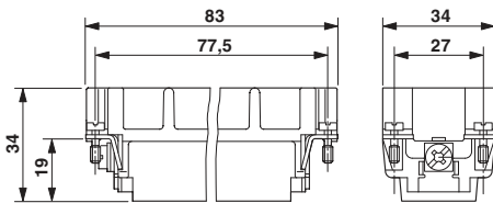
Dimensioned drawing
