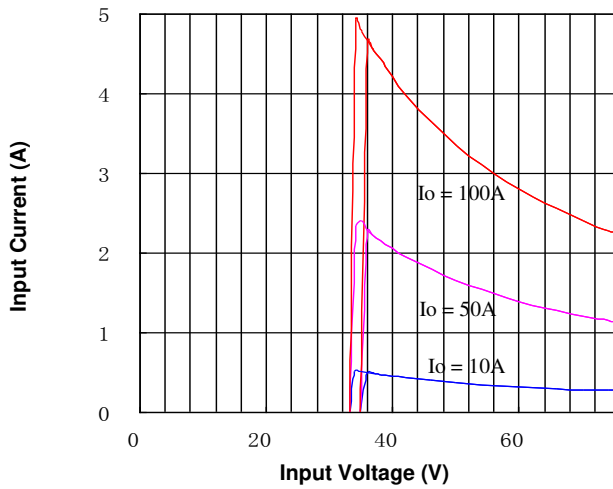
Figure 7. Input Characteristics
