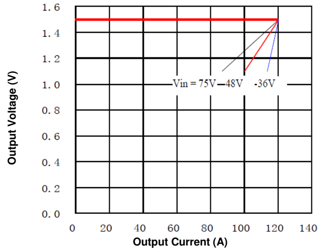
Figure 8. Output Characteristics
