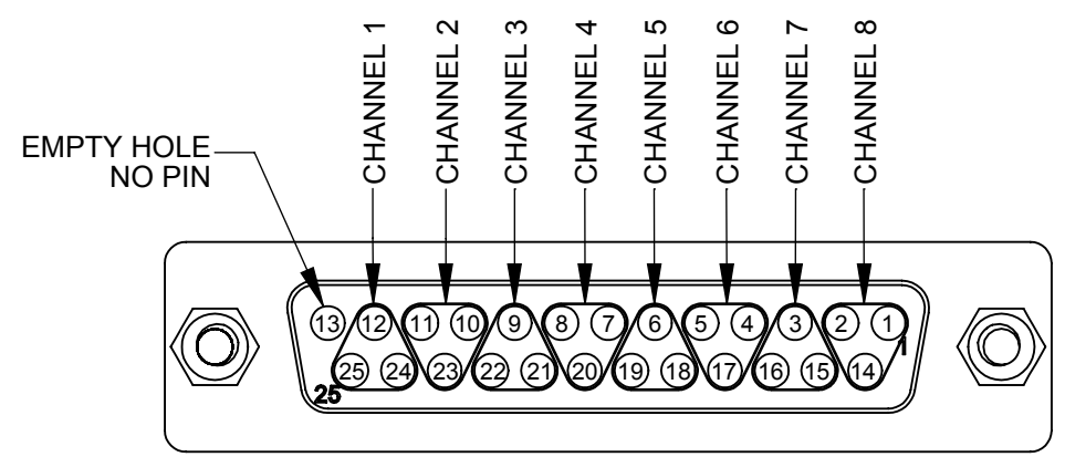
DB25F PIN-OUT VIEW
