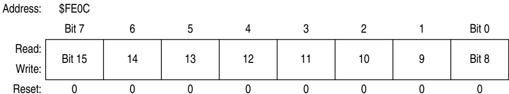
Figure 21-4. Break Address Register High (BRKH)
