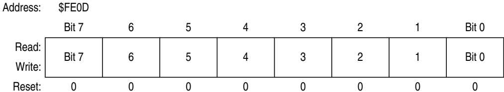
Figure 21-5. Break Address Register Low (BRKL)
