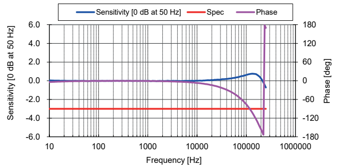
Figure 12: Frequency response
