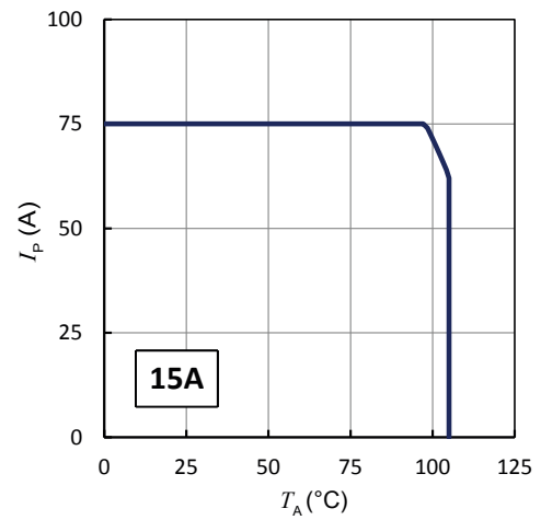
Figure 17: I_p vs T_A for HO series
