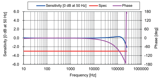
Figure 7: Frequency response
