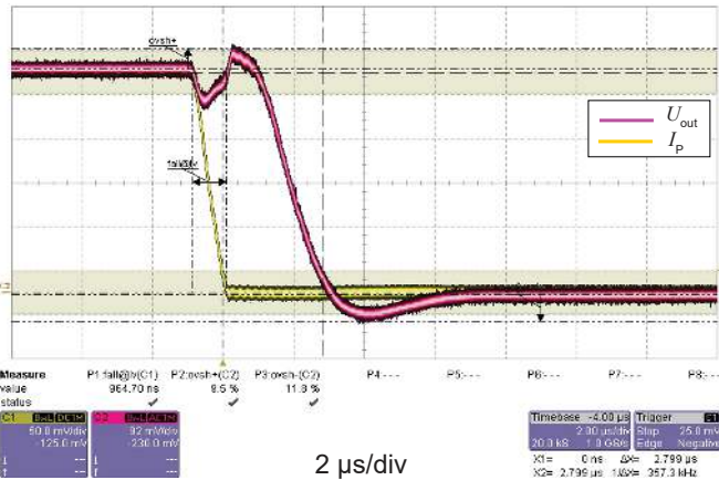
Figure 13: Step response
