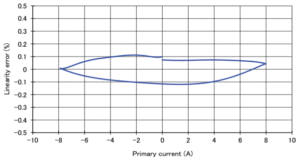
Figure 1: Linearity error
