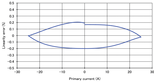
Figure 11: Linearity error
