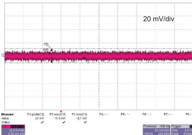
Figure 15: Output noise
