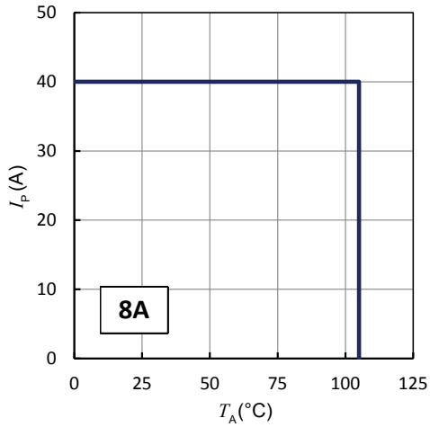
Figure 16: I_p vs T_A for HO series
