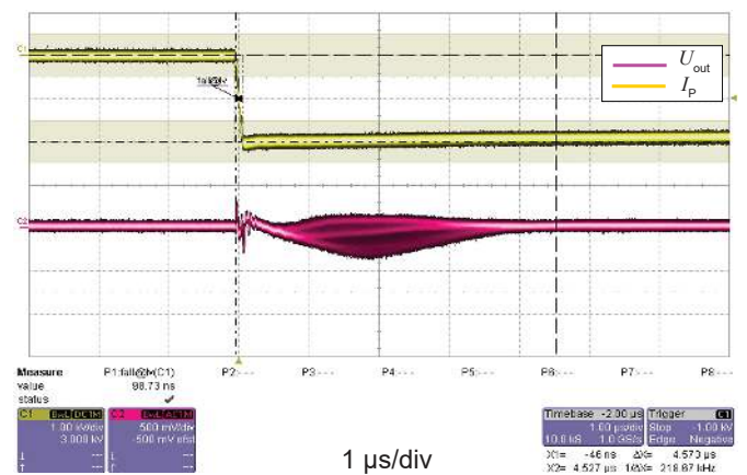
Figure 14: dv/dt
