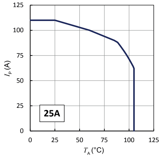
Figure 18: I_p vs T_A for HO series
