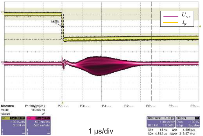
Figure 4: dv/dt
