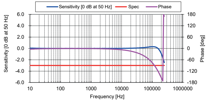
Figure 2: Frequency response
