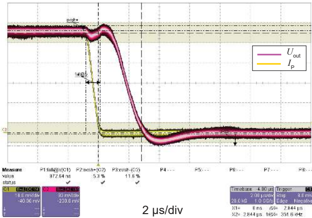
Figure 3: Step response
