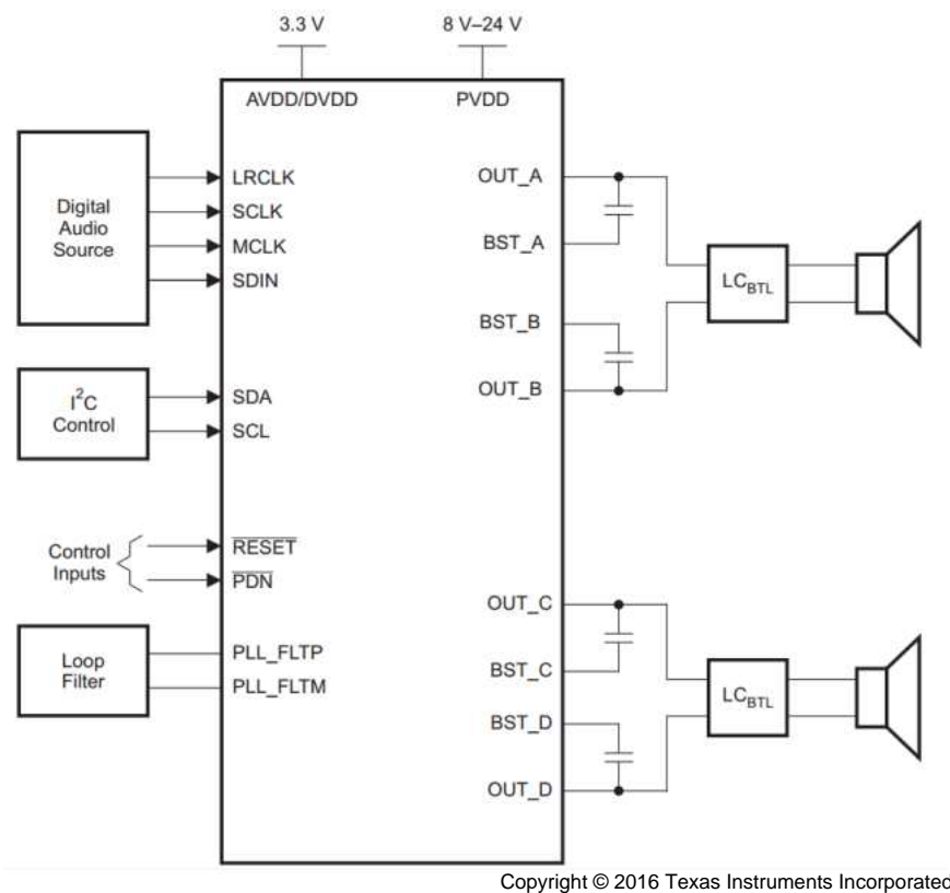
Figure 40. TAS5727 Stereo Application
