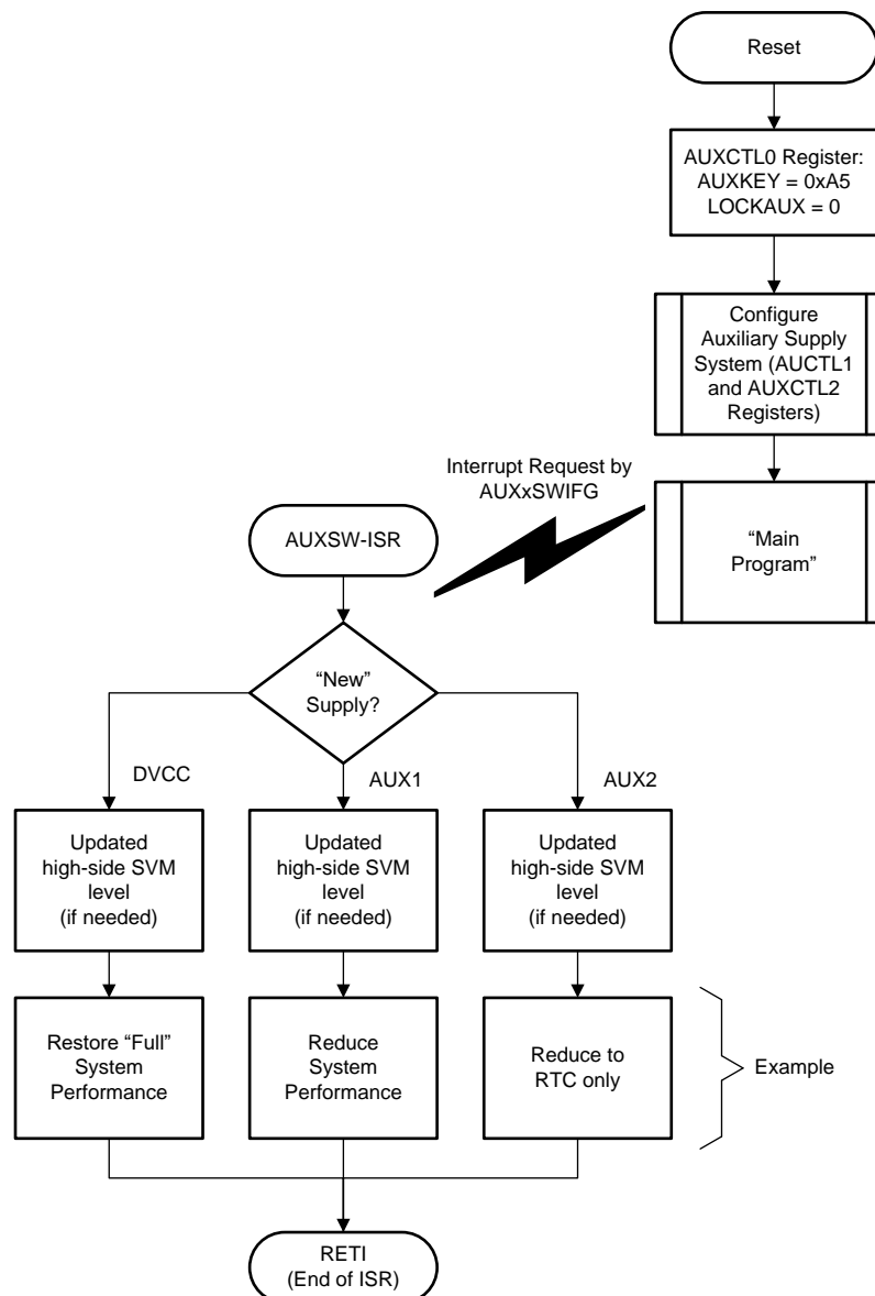
Figure 4-9. Software Flow Chart
