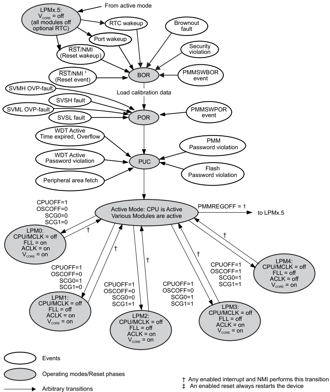
Figure 1-6. Operation Modes
