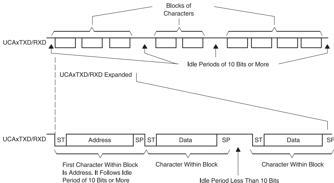
Figure 36-3. Idle-Line Format
