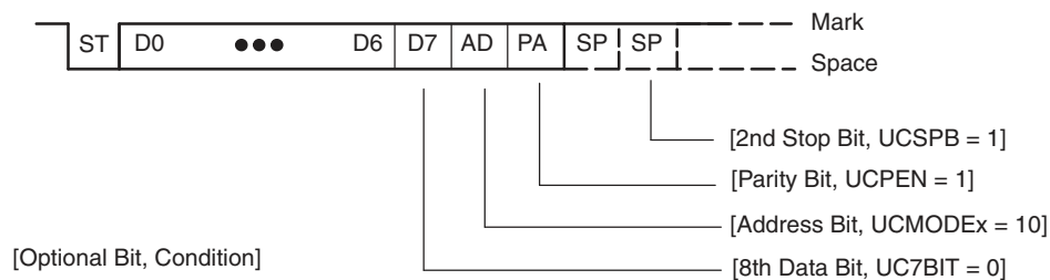
Figure 36-2. Character Format
