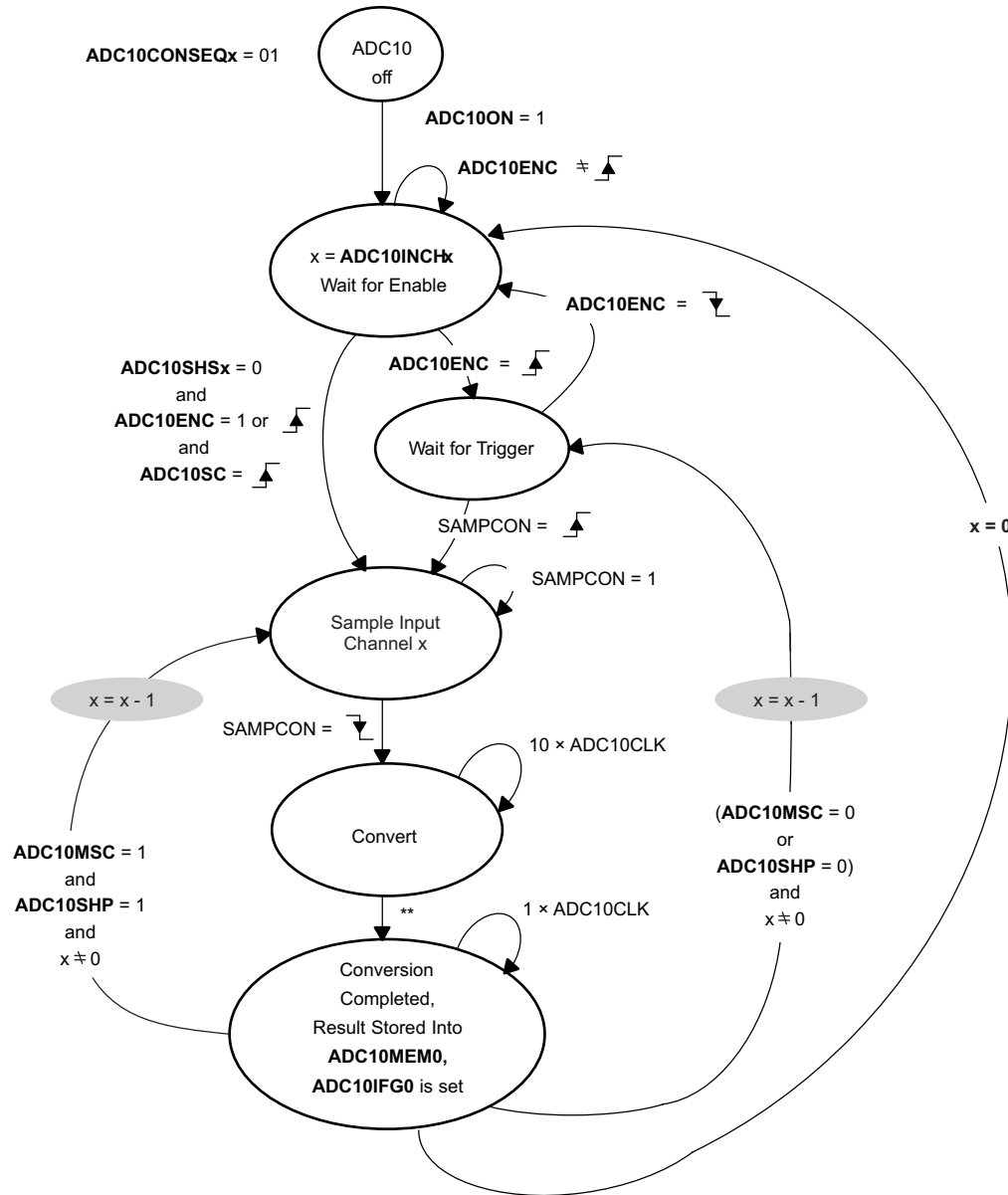
Figure 27-7. Sequence-of-Channels Mode
