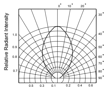
FIG.5 Radiant Diagram
