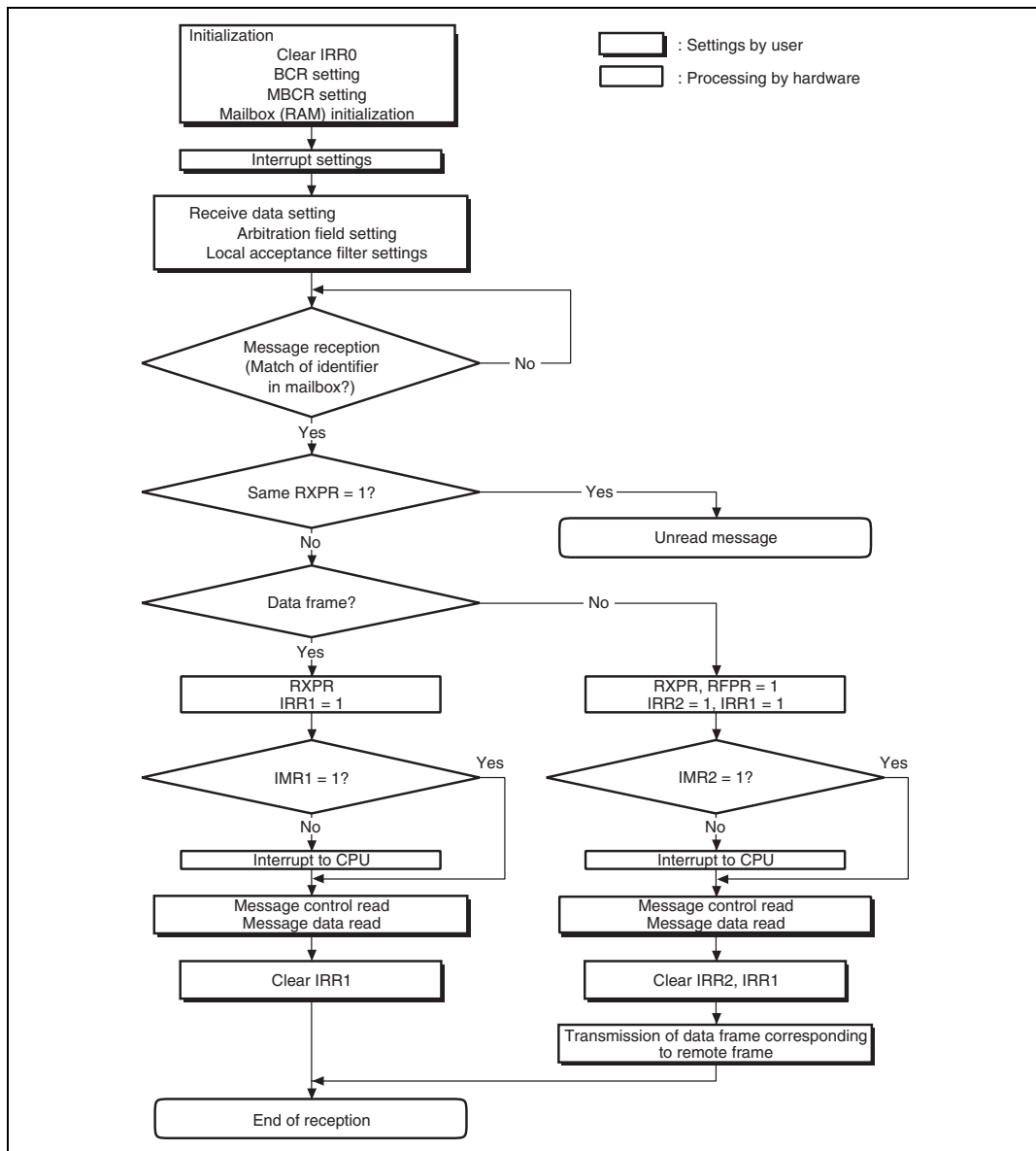
Figure 15.11 Reception Flowchart
