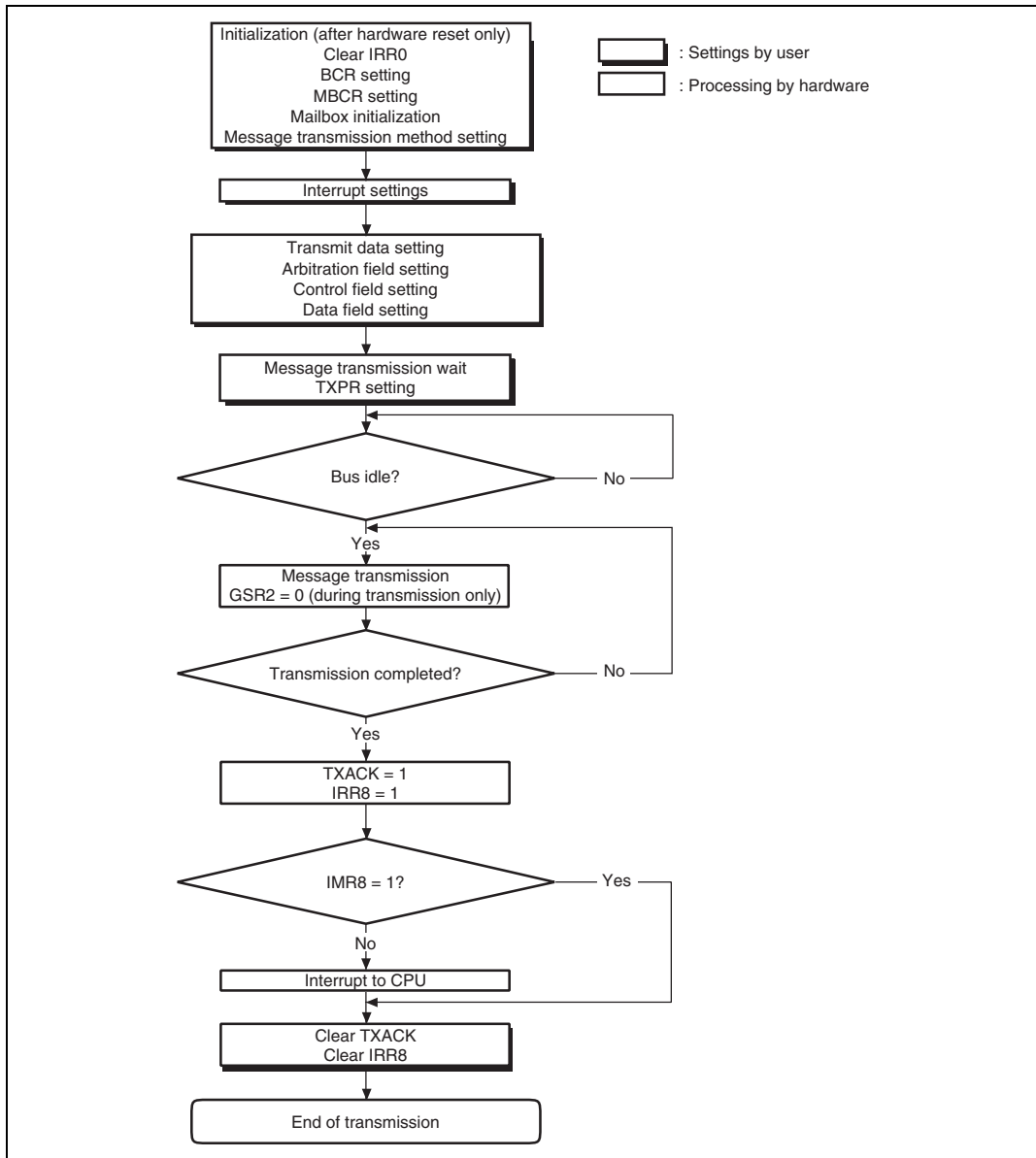
Figure 15.9 Transmission Flowchart
