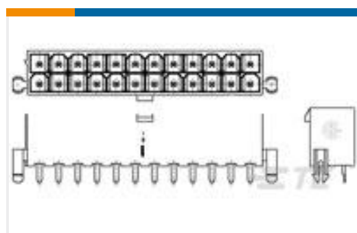
TE Part #2-1586039-4 24P VAL-U-LOK VRT HDR W/P V2
