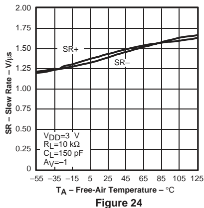
SLEW RATE vs FREE-AIR TEMPERATURE
