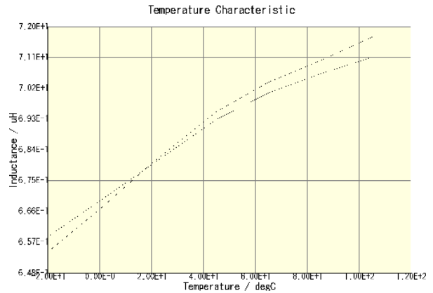
CLF7045T-680M-CA(DC = 0A)
