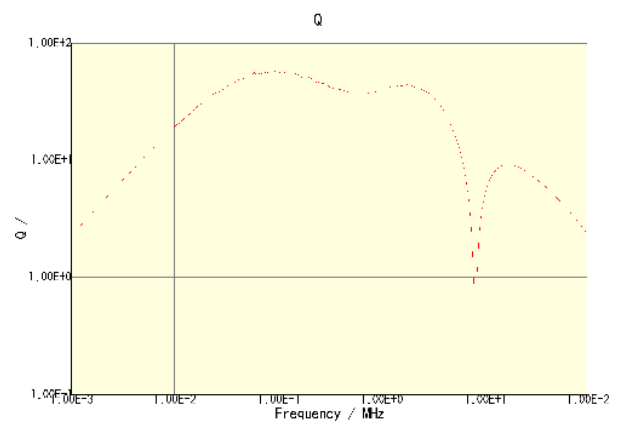
CLF7045T-680M-CA
