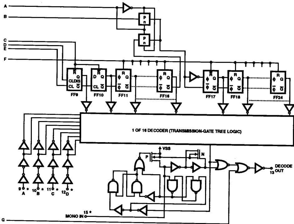
DETAIL FOR FF9, 11-16, 17-24
