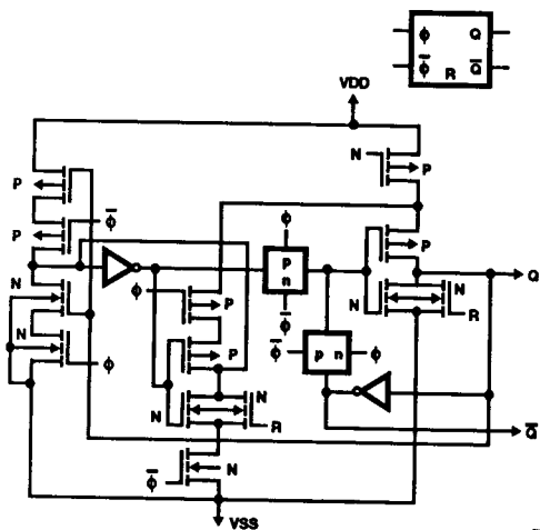
DETAIL FOR FF9, 11-16, 17-24
