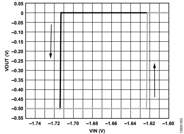
Figure 49. Typical UVLO Behavior, V_{OUT} = -0.5 \text{ V}
