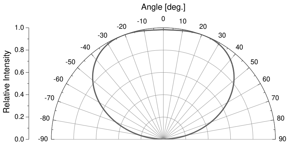
Fig 8. Typical Angular Diagram, I_F=150\text{mA}
