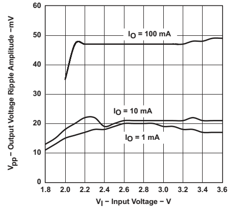
Figure 14. Output Voltage Ripple Amplitude vs Input Voltage
