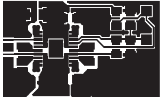
Figure 19. Recommended Component Placement and Board Layout
