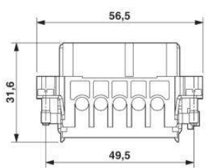
Female insert
