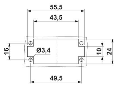
Panel cutout
