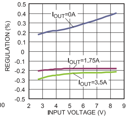
Line Regulation (PSM)
