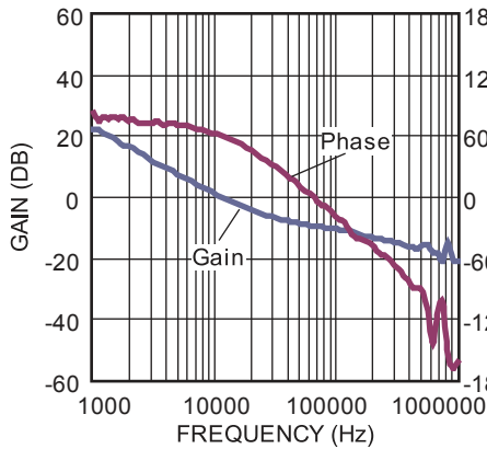
Bode Plot
