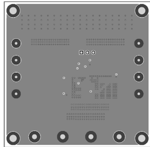
Figure 4—Inner Layer 2
