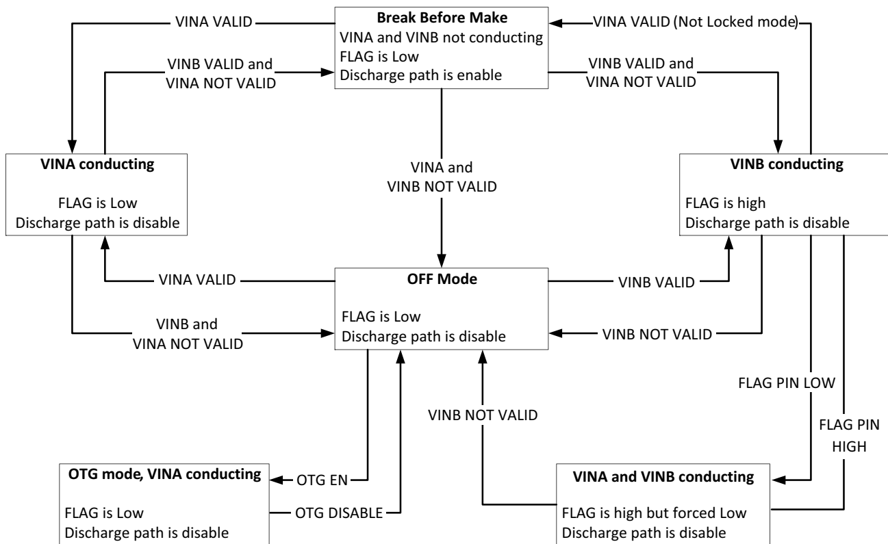
Figure 8. Functional Diagram
