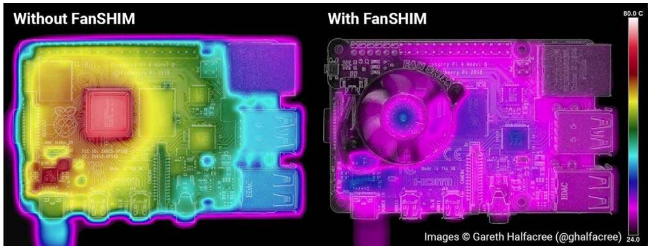
Thermal images of Raspberry Pi 4 with and without FanSHIM installed. Images by Gareth Halfacree - check out his full benchmark blog post.
