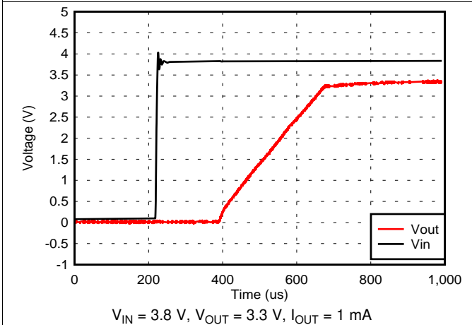
Figure 23. V_{IN} Power-Up
