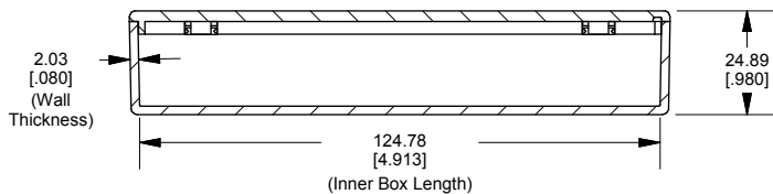
SECTION B-B
