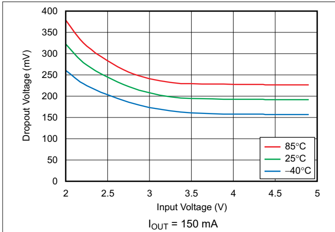
Figure 6-13. Dropout Voltage vs Input Voltage
