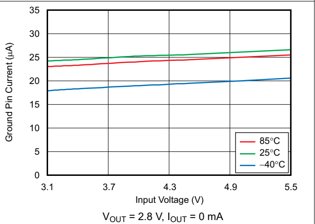
Figure 6-18. Ground Pin Current vs Input Voltage
