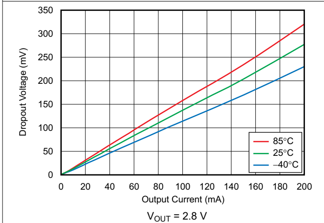
Figure 6-15. Dropout Voltage vs Output Current
