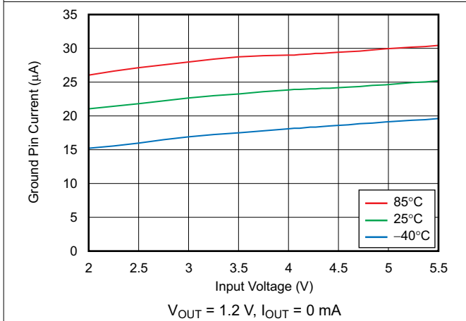
Figure 6-17. Ground Pin Current vs Input Voltage
