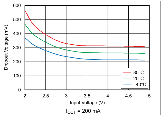
Figure 6-14. Dropout Voltage vs Input Voltage
