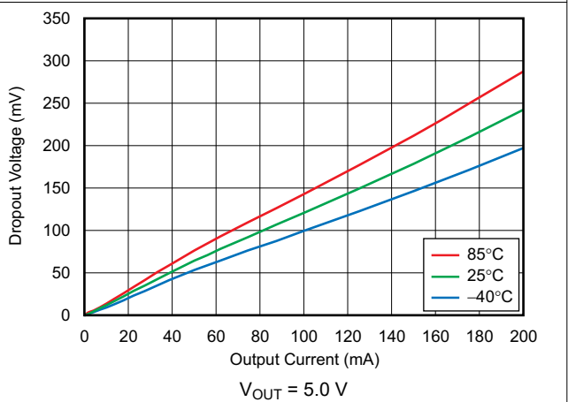
Figure 6-16. Dropout Voltage vs Output Current
