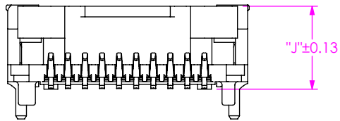
FIG 4 PICK AND PLACE PAD UCC8-010-1-XXX-S-1-A SHOWN (DIFFERENT AS SHOWN, OTHERWISE SAME AS FIG 1; USE PPP-73-XXX FOR BOTH -1 & -2 WELD TAB LEAD STYLES)
