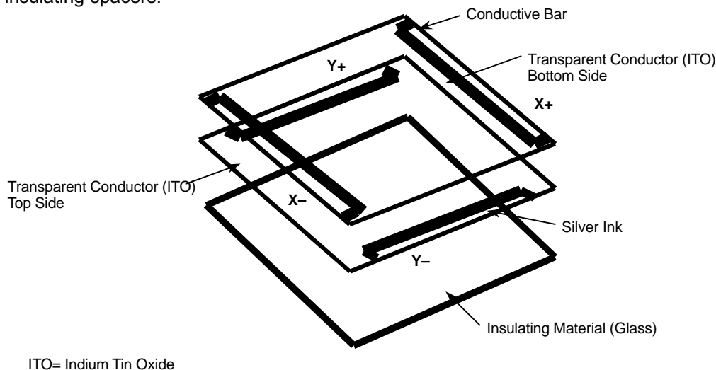
Figure 40. 4-Wire Touch Screen Construction
