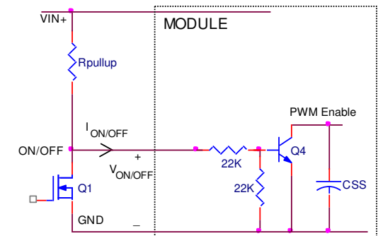
Figure 40. Circuit configuration for using negative On/Off logic.
